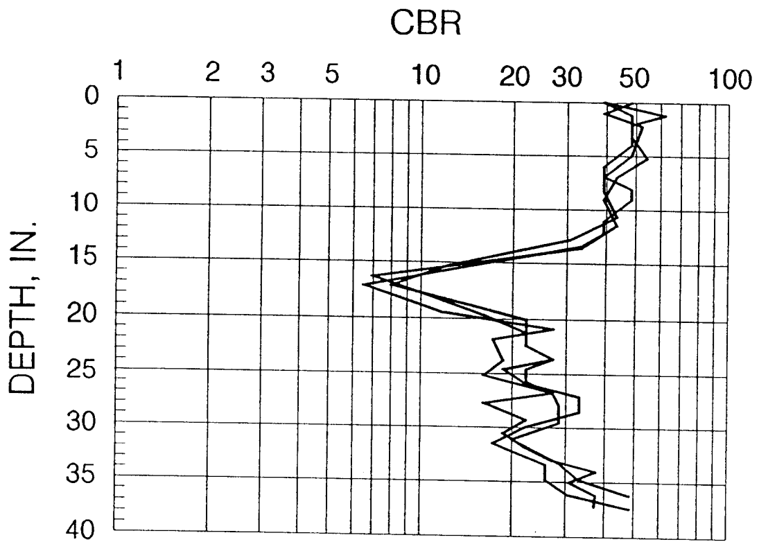
Figure 11. Example of DCP data plot for three tests in similar type soils
