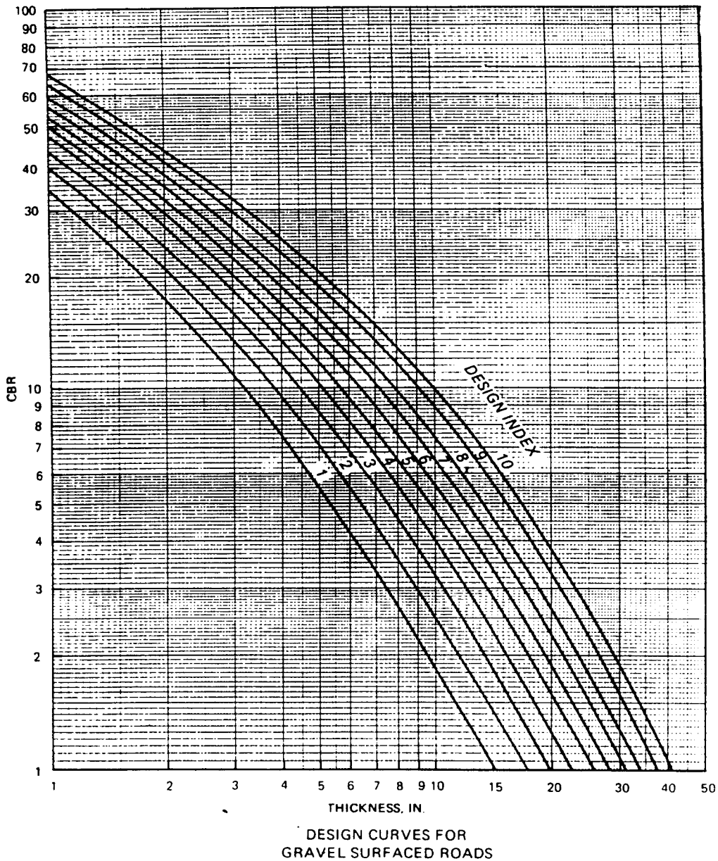
Figure 1. Thickness design curves for aggregate surfaced roads.
